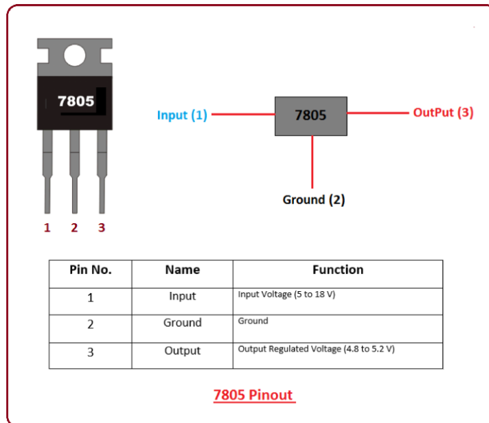
Fig 8 pinout of 7805
