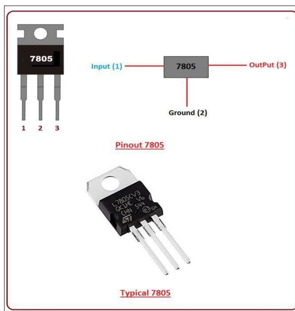
Fig 7 7805 voltage regulator
