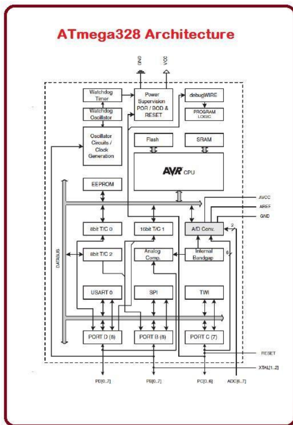
Fig 4 ATmega328 architecture
