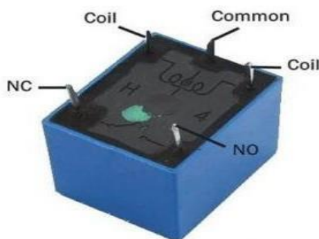
Fig 15 5V Relay
