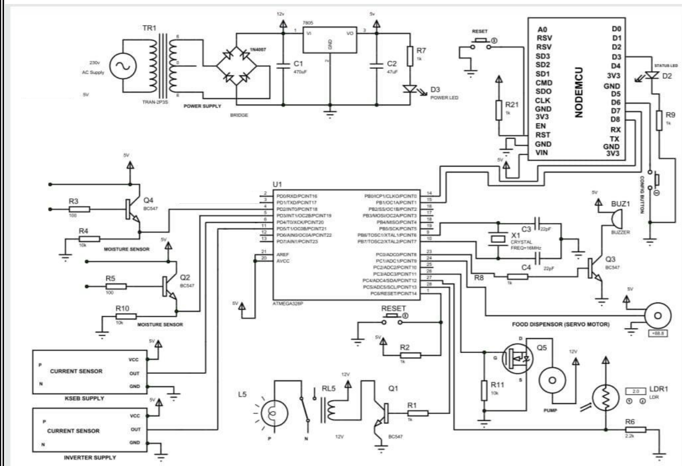
Fig 21 circuit diagram
